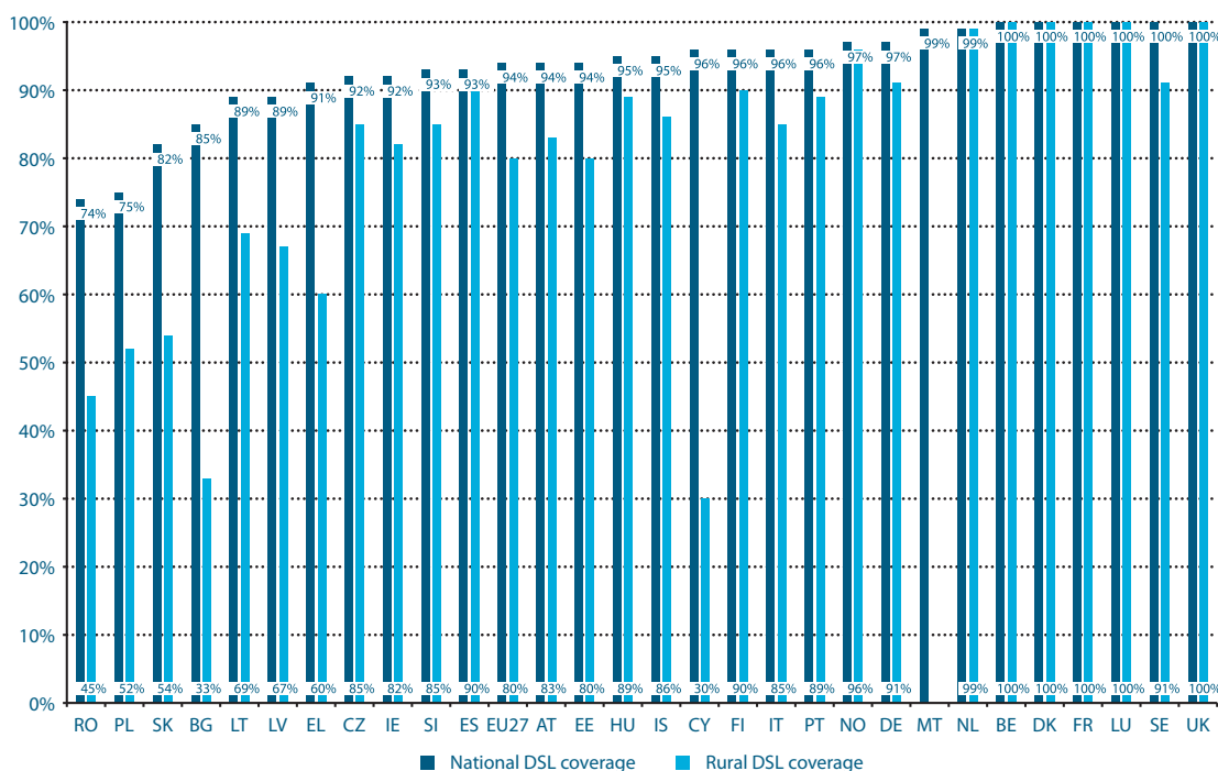
Figure 2.16: DSL national and rural coverage, December 2009
